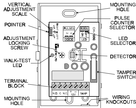
Figure 7. Printed Circuit Board
