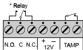
Figure 6. Terminal Block
